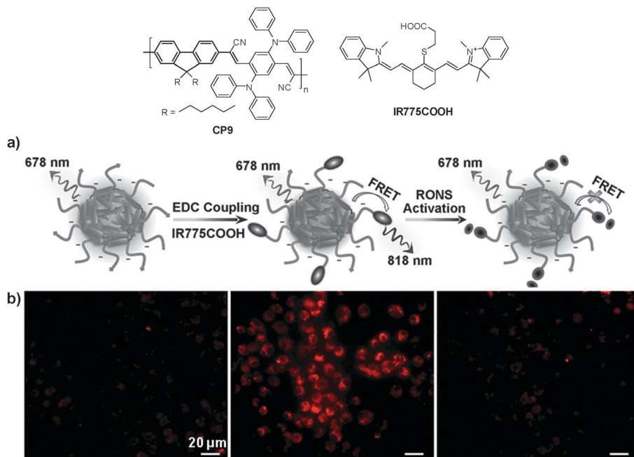
Fig. 8 Chemical structures of CP9 and IR775COOH . (a) Schematic illustration of RON detection using CP9 /IR775 FRET nanoparticles. (b) Fluorescence images of live murine macrophages (RAW 264.7) incubated with CP9 /IR775 nanoparticles. From left to right: untreated cells, cells successively treated with LPS and PMA, and cells pre-treated with NAC before incubation with LPS and PMA, followed by NAC treatment. All the images share the same scale bar of 20 μm (reprinted with permission from ref. 96, Copyright 2013 Wiley-VCH).
