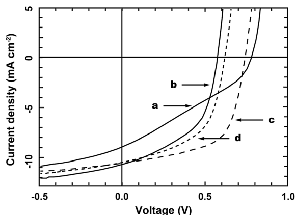
Fig. 26 Current density vs. voltage ( J - V ) curves under 100 \text{ mW cm}^{-2} air mass 1.5G simulated solar illumination, of (a) ITO/MoO 3 / 286 :C 60 /C 60 /BCP/Ag; (b) ITO/MoO 3 /FDTS/ 286 :C 60 /C 60 /BCP/Ag; (c) ITO/MoO 3 / 286 (105 °C)/C 60 /BCP/Ag; and (d) ITO/MoO 3 /FDTS/ 286 (105 °C)/C 60 /BCP/Ag. (Reproduced with permission from ref. 144. Copyright 2010, Elsevier B.V.)
