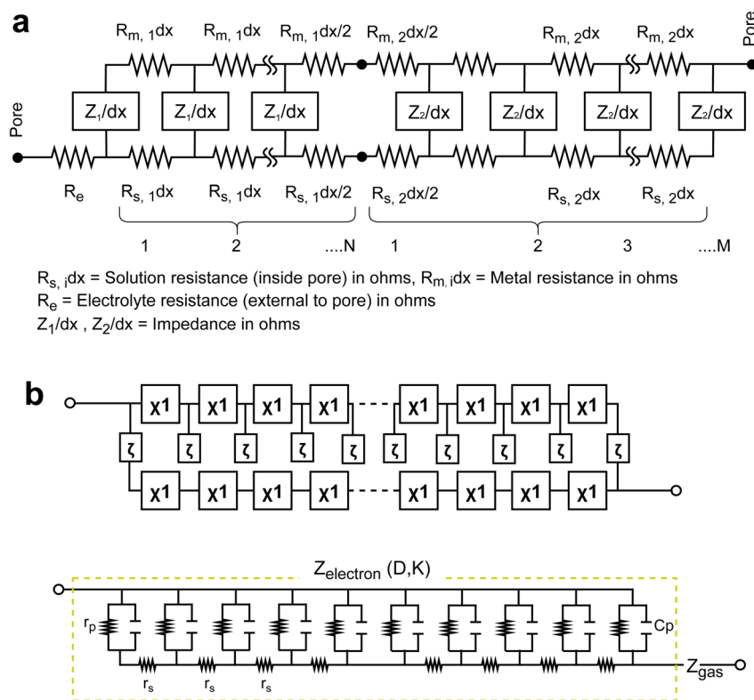
Fig. 14 Representative porous-electrode transmission-line schematics used to describe distributed impedance in porous systems: (a) a detailed pore model including electrolyte resistance external to the pore ( R_e ), solution resistance inside the pore ( R_{s,1}dx ), metal resistance ( R_{m,1}dx ), and distributed local impedance elements ( Z_1/dx , Z_2/dx ). Reproduced from ref. 381 with permission from IOP Publishing, copyright 2009; and (b) a simplified ladder-network representation highlighting distributed ionic/electronic pathways and interfacial contributions, including pore resistance ( r_p ), series resistance ( r_s ), pore capacitance ( C_p ), and terminal impedance terms Z_{\text{electron}}(D, K) and Z_{\text{gas}} . Reproduced from ref. 382 with permission from the Korean Ceramic Society, copyright 2016, under CC BY-NC 4.0 ( http://creativecommons.org/licenses/by-nc/4.0/ ). These schematics illustrate how porous-electrode architectures naturally generate distributed impedance responses, motivating porous-electrode-aware interpretation of Nyquist features.
