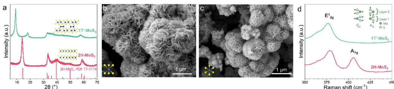
Fig. 1 (a) XRD patterns of 2H- and 1T'-MoS 2 ; (b and c) SEM images of 2H- and 1T'-MoS 2 ; (d) Raman spectra of 2H- and 1T'-MoS 2 .
