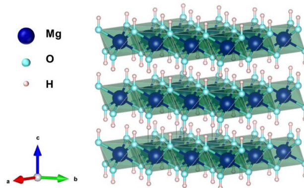
Fig. 1 Crystal structure of brucite ( Mg(OH)_2 ) (reprinted with permission from ref. 21 Copyright 2022 MDPI, Basel, Switzerland, under the terms and conditions of the Creative Commons Attribution (CC BY) license).
