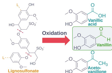
Fig. 1 Oxidative depolymerization of a lignosulfonate substructure (linked to a larger lignin polymer, L) into three common products. Cleavable bonds are shown as red dashed lines.
