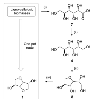
Fig. 14 One-pot isosorbide synthesis starting from biomasses. 15
