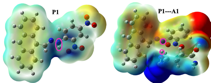
Fig. 14 Electrostatic potential plots of probe P1 and complex ( P1 · A1 ), generated at the CAM-B3LYP/6-31+G(d,p) level of theory using the CPCM-DMSO solvation model. The pink color represents the atoms involved in the proton shift.
