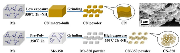
Fig. 7 Synthesis procedure of porous GCN using a pre-polymerization method. Inset: SEM image of porous GCN. Reprinted with permission from ref. 64 Copyright 2018, Elsevier.
