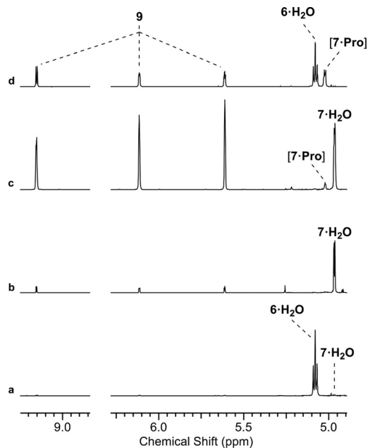
Fig. 3 Proline-catalysed aldol-elimination cascade. (a) 1 H NMR [400 MHz, noesygprrld, H 2 O/D 2 O (9 : 1)] spectrum to show the reaction of glycolaldehyde phosphate ( 6 , 100 mM) with formaldehyde ( 8 , 100 mM) in phosphate buffer (500 mM, pH 7) at 40 °C after 48 h; (b and c) 1 H NMR [700 MHz, noesygprrld, H 2 O/D 2 O (9 : 1)] spectra to show the reaction of glyceraldehyde-2-phosphate ( 7 , 100 mM) in phosphate buffer (500 mM, pH 7) with 50 mol% L- Pro at 40 °C after: (b) 0.5 h; (c) 48 h; (d) 1 H NMR [400 MHz, noesygprrld, H 2 O/D 2 O (9 : 1)] spectrum to show the reaction of 6 (100 mM) with 8 (100 mM) in phosphate buffer (500 mM, pH 7) with 50 mol% L- Pro at 40 °C after 7 h.
