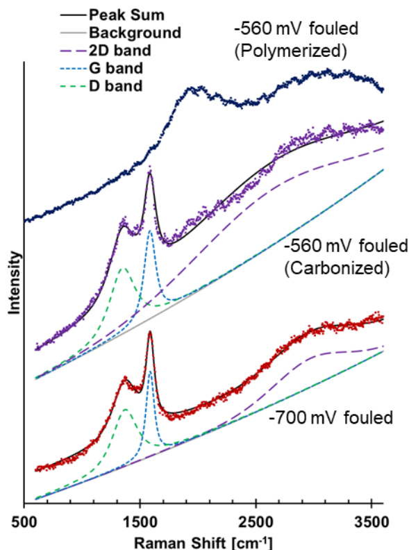
Figure 6. Raman spectra of -700 mV RHE fouled Cu showing D, G, and 2D bands, spectra of -560 mV RHE fouled Cu showing spectra from a carbonized area of electrode and a polymerized area of the electrode.
