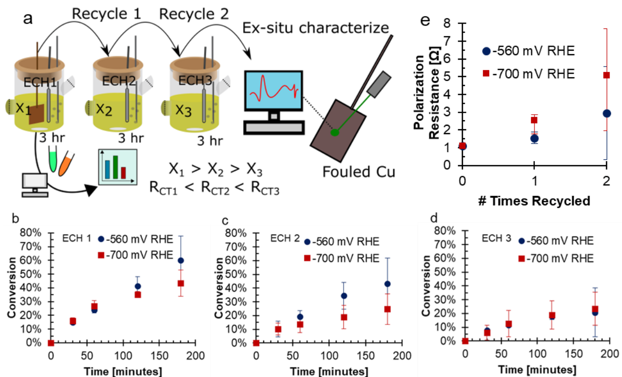
Figure 1. (a) A schematic showing the experimental procedure of this work, noting that the ECH cell depicts only the cathodic chamber while a full cell was used as depicted in 17 . Conversion of FF during 3 hour ECH with recycle showing (b) ECH1, (c) ECH2 (d) ECH3. Conditions: 200 mM FF, 0.5 M H 2 SO 4 , 80:20 vol% water:acetonitrile, 60 mL N 2 sparging, 25 °C, Cu electrode. (e) Polarization resistance before ECH determined using EIS. X-axis shows the number of uses prior to the EIS. EIS conditions: -560 mV RHE RMS, 10 mV amplitude, 0.1 Hz to 100kHz.
