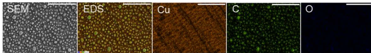
Figure 5. SEM/EDX images at 5000x magnification for a Cu foil electrode submerged into catholyte solution containing 100 mM of FF and 30 mM of FA for 3 hours. Scale bar shown is 10 \mu\text{m} .
