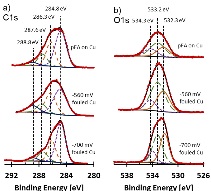
Figure 7. C1s and O1s XPS spectra for pFA on Cu, -560 mV RHE fouled Cu, and -700 mV RHE fouled Cu. Vertical dotted lines mark the assignments for C1s and O1s spectra for deconvolution.
