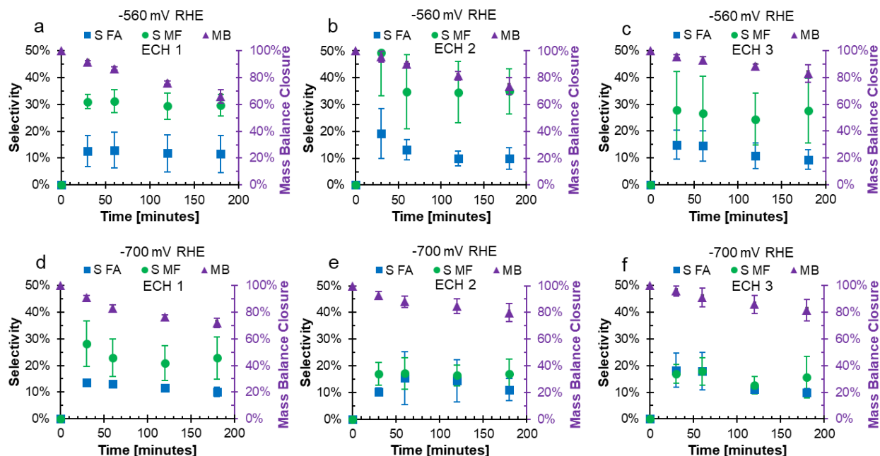
Figure 2. Mass balance and selectivity to FA and MF from consecutive ECH of FF with recycled Cu foil electrode. At -560 mV RHE: (a) ECH1, (b) ECH2, (c) ECH3. At -700 mV RHE: (d) ECH1, (e) ECH2, (f) ECH3. Conditions: 200 mM FF, 0.5 M H 2 SO 4 , 80:20 vol% water:acetonitrile, 3 hour duration ECH, 60 mL N 2 sparging, Cu electrode.
