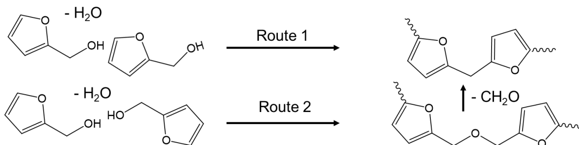
Scheme 1. Reaction pathway for pFA formation from FA in acid.
