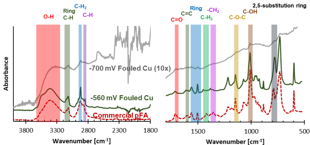
Figure 4. FTIR spectra of -560 mV RHE fouled Cu polymer, commercial pFA, and 10x magnified -700 mV RHE fouled Cu. Shaded areas indicate key pFA bands summarized in Table S3.
