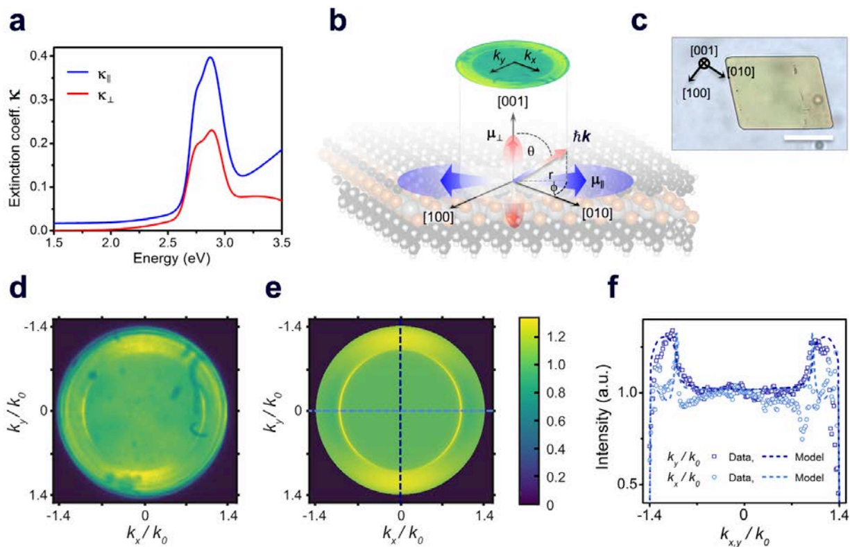
Figure 3. Experimental assessment of the in-plane \hat{\mu}_{\parallel} and the out-of-plane \hat{\mu}_{\perp} excitonic dipole moments. a , Optical extinction coefficient \kappa for the in-plane \kappa_{\parallel} and out-of-plane \kappa_{\perp} components, calculated from ellipsometry fit indicating a strong anisotropy. b , Schematic of exciton transition dipole orientation \hat{\mu} within the crystal derived from ellipsometry and PL experiments; projection of the PL photon momentum onto the Fourier plane as detected by back focal plane imaging (BFP). c , Optical image of the micron-size single crystal. Scale bar, 20 \mu\text{m} . d-f , BFP image and modelling of single crystal PL directionality. Experimental ( d ) and modelled ( e ) back focal plane image for the emission from a single crystal through a linear polariser aligned with the [010] axis. The \hat{\mu}_{\parallel} strength is 1.7\times higher on average than the \hat{\mu}_{\perp} strength, as described by the modelling of the horizontal (light blue) and vertical (dark blue) cross sections ( f ).
