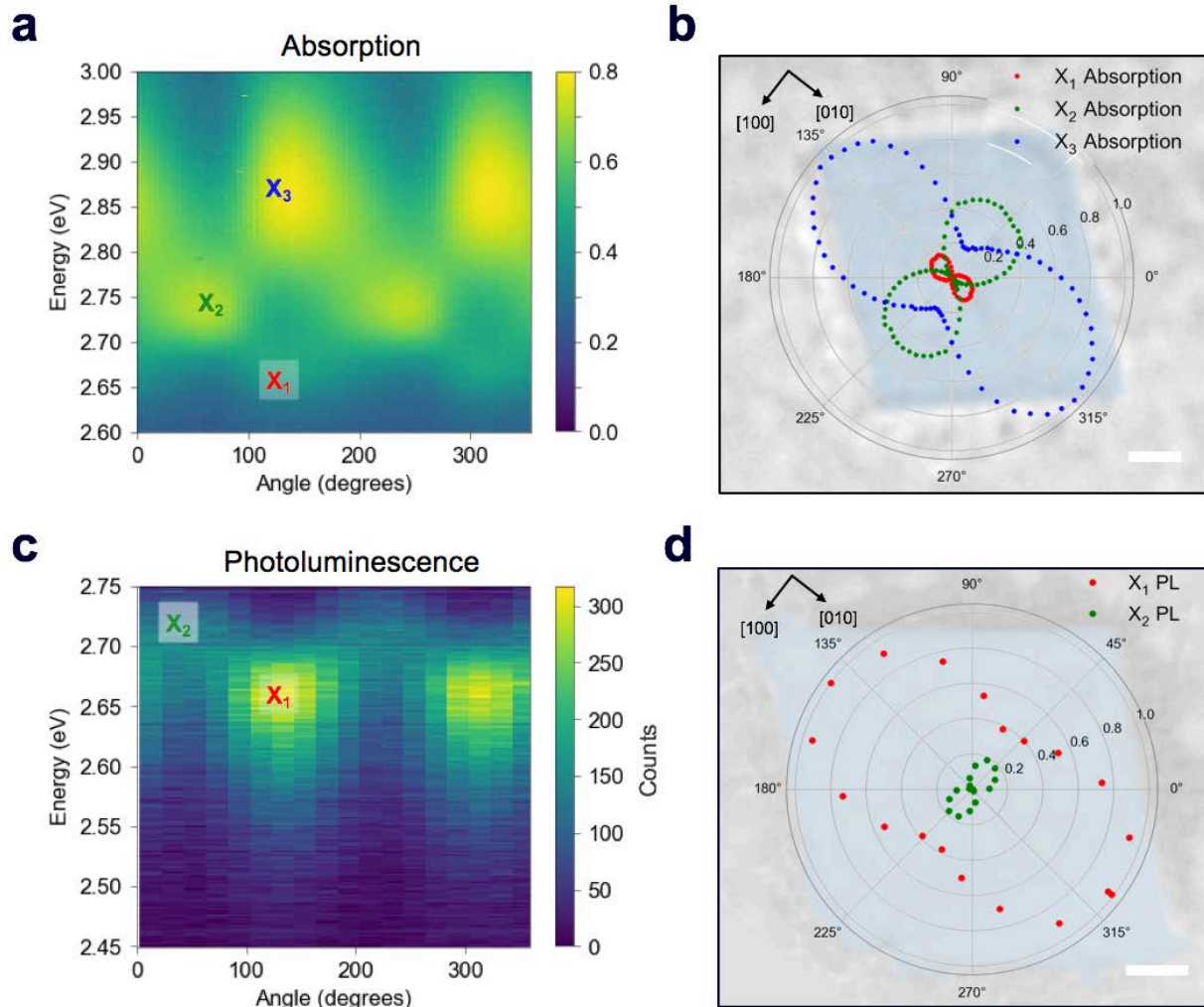
Figure 4. The in-plane anisotropy of the energy-resolved dipole moments. Angle-resolved absorption spectra (a) and PL spectra (c) for different linear polarizations of the incident light (a) and emitted light (c) are shown. Excitons X 1 and X 3 contribute to \hat{\mu}_{[010]} while X 2 contributes to the orthogonal \hat{\mu}_{[100]} . PL was only detectable from X 1 and X 2 in our system. The fitted intensities of the absorption peaks (b) and PL peaks (d) are plotted in polar coordinates and overlaid to the measured crystal to give spatial coordinate reference. Scale bars, 5 μm.
