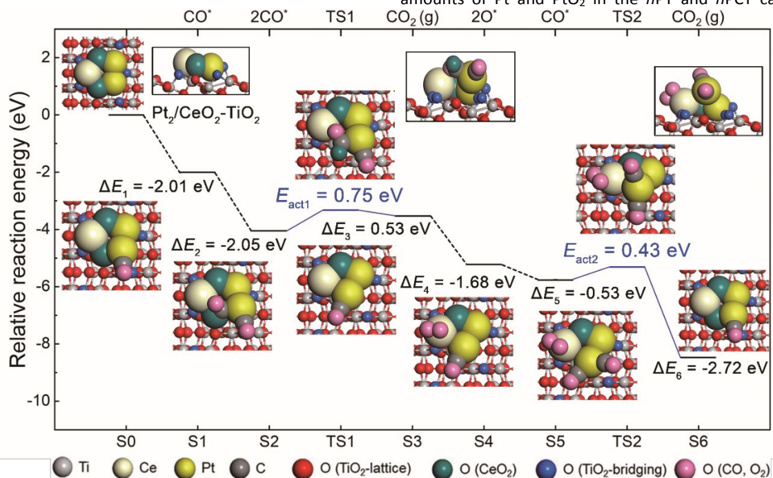
Fig. 4 DFT-predicted MvK-type CO oxidation pathway catalyzed by a \text{Pt}_2 cluster pinned at the \text{CeO}_x\text{-TiO}_2 interface. \Delta E_n denotes the relative energy of the n^{\text{th}} stage with respect to the (n-1)^{\text{th}} stage. For example, \Delta E_3 was calculated as follows: \Delta E_3 = \text{Energy of stage 3} .
