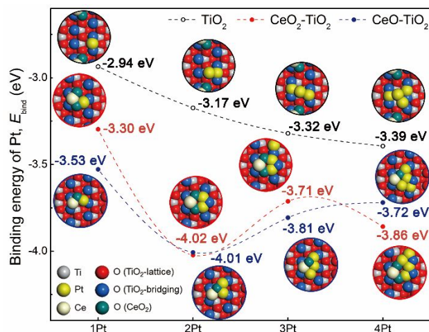
Fig. 1 DFT-calculated binding trend of Pt-SAs on TiO 2 (101) and at the CeO 2 -TiO 2 interface with fully oxidized or reduced Ce ions. The E_{\text{bind}} of n\text{Pt} represents the average binding energy of total number of Pt atoms.
