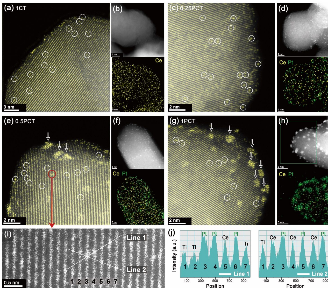
Fig. 2 Morphology of \text{CeO}_x\text{-TiO}_2 support and n\text{PCT} catalysts ( n \leq 1 ). (a) High-angle annular dark-field (HAADF)-STEM images of \text{CeO}_x\text{-TiO}_2 supporting oxide with 1 wt.% initial Ce-loading. (b) HAADF-STEM and Ce EDS scan images of the \text{CeO}_x\text{-TiO}_2 presented in (a). HAADF-STEM image and Ce and Pt EDS scan image of 0.25PCT [(c) and (d)], 0.5PCT [(e) and (f)], and 1PCT [(g) and (h)]. Atomic-sized bright spots in (c), (e), and (g) denote Pt-SAs and \text{CeO}_x clusters. Some of the \text{CeO}_x clusters and Pt-SAs are highlighted in white circles. Ce and Pt EDS scan images [(d), (f), and (h)] confirm the locational correlation of \text{CeO}_x and Pt-SAs on \text{TiO}_2 powder surfaces. (i), (j) Intensity profile of the selected highlighted area of 0.5PCT, which clearly show the intimate contact between Pt, Ce, and Ti ions. Arrows in (e) and (g) indicate Pt NPs formed under the higher Pt-loading.
