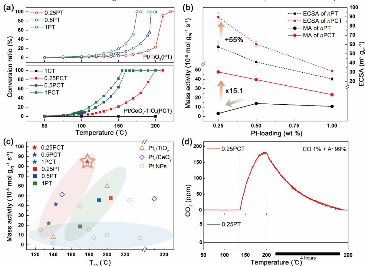
Fig. 5 CO oxidation performance of n Pt and n PCT catalysts. (a) Temperature-programmed CO conversion profile (light-off curve) of n Pt and n PCT catalysts. (b) The specific mass activity (MA) of n Pt and n PCT catalysts at 140 °C as a function of Pt-loading and the ECSA of n Pt and n PCT catalysts. The MA of n PCT catalysts is an inverse function of Pt-loading, whereas the MA of 0.25PT is lower than the others. (c) The specific MA values of n Pt and n PCT catalysts plotted as a function of T_{50} . Reference values were limited to Pt-SAs or NPs supported on conventionally synthesized or purchased CeO 2 or TiO 2 . (refer to ESI† for the full reference list). (d) CO-TPR analysis results of 0.25PT and 0.25PCT catalysts.
