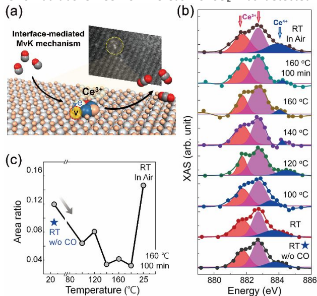
Fig. 6 Operando gas phase XAS analysis. (a) Schematic diagram of Ce reduction upon CO oxidation by the MvK mechanism at the Pt- \text{CeO}_x\text{-TiO}_2 interface. (b) Operando XAS with respect to reaction temperatures. Owing to low signal-to-noise ratio, XAS was obtained from entire particle region. De-convoluted spectral features for \text{Ce}^{3+} (red and magenta shaded areas, energy positions are indicated as red arrows) and \text{Ce}^{4+} (blue shaded area, energy positions are indicated as blue arrow) are superimposed on averaged XAS. (c) Area ratio between de-convoluted spectral features of \text{Ce}^{3+} and \text{Ce}^{4+} in (b).
