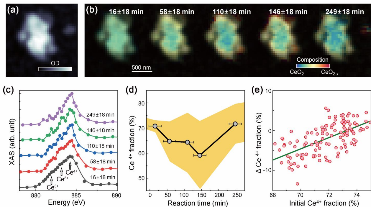
Fig. 3 Electronic interaction between Pt and Ce upon formation of Pt-SAs at the CeO x -TiO 2 interfaces, which is directly observed by operando X-ray absorption spectroscopy. (a) Averaged optical density map across Ce M 5 -edge. (b) Spatio-temporal chemical evolutions with respect to reaction time. Chemical phase maps obtained by linear combination fits of XAS data at each pixel (see Methods in the ESI † ). The fitting results (chemical information) and averaged optical density (morphological information) are presented by color legend and transparency, respectively. The presence of CeO 2 and CeO 2-x , assigned colors blue and red, respectively. (c) Operando XAS from entire particle region in (a). Energy positions of M 5 -edge absorption features for Ce 3+ and Ce 4+ are indicated as black arrows. (d) Ce 4+ fraction versus reaction time. Scatters and yellow shaded area indicate average and standard deviation of Ce 4+ fraction from entire particle region, respectively. The error range of the reaction time is estimated by the liquid injection time (see Methods in the ESI † ). (e) Distribution plot for initial Ce 4+ fraction versus fraction difference between the first and second measurements (solid red scatters). Solid green line is a guide to eye.
