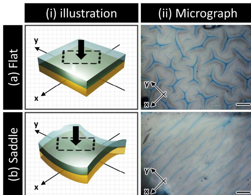
Figure 4| Experimental demonstration of the mechanical coupling of surface crease pattern with the saddle-like bending. Different surface crease patterns were formed for the hydrogel sheets fixed onto a flat substrate (a) and saddle-shaped substrate (b). Column (i) is a schematic illustration of the hydrogel-coated unswellable substrate, where the blue part represents the hydrogel sheet (thickness: 500 \mu\text{m} ), while the yellow part indicates the polyurethane rubber which is the unswellable substrate. The micrographs presented in column (ii), observed with an optical microscope, show the surface morphology of the gel. In order to observe clearly the boundary of the surface pattern, the coated hydrogel sheets were swollen in water containing 0.05 wt % Alcian blue. After reaching the equilibrium state ( \sim 600 s), isotropic polygonal-like pattern and anisotropic straight-grained pattern were observed on the surface of (a-ii) and (b-ii), respectively. All the micrographs have the same scale bar (500 \mu\text{m} ). After swelling, the thickness of gel reached to 1.15 mm. The curvature of saddle is 0.155 [1/mm].
