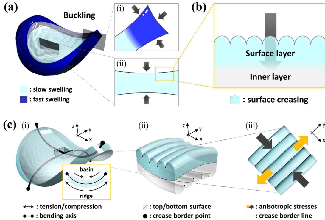
Figure 3| Schematic illustration of two kinds of swelling mismatch and their coupling to induce anisotropic surface creases during fast free swelling of a polyelectrolyte gel. (a) Swelling mismatch between the annulus (dark blue) and the inner disc (light blue) induced by the difference in swelling kinetics between the annulus and the inner disc. The annulus can absorb water from three directions (a-i), while the inner disc can only absorb water from two directions (a-ii) as shown by arrows in (a-i, ii). This swelling mismatch induces a saddle-like bending to minimize the swelling mismatch. (b) Swelling mismatch between the surface layer (light blue) and inner layer (gray) induced by the difference in swelling kinetics between the surface layer and the inner layer. Surface creasing instability is induced to minimize this swelling mismatch. (c) The two mechanical instabilities are coupled to induce anisotropic surface crease pattern. Bending of the sample exerts a tension to the ridge and a compression to the basin (c-i). The saddle-like bending induces anisotropic stresses, perpendicularly oriented, on the two surfaces of the sample (c-ii), which changes the isotropic polygonal crease patterns into the anisotropic stripe crease patterns aligned in right angles on the two surfaces (c-iii).
