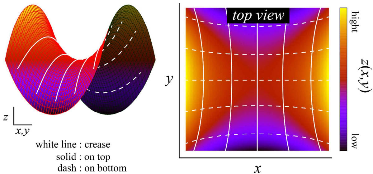
Figure 6| Creases on the Scherk's minimal surface. The colored surface is the Scherk's minimal surface, and the solid and dashed lines represent the creases of the top and bottom surfaces, respectively. These lines are the orbits obtained by the calculation of the differential equation from Eq. 6. On any intersection, these lines are at right angles to each other when viewed from the normal direction.
