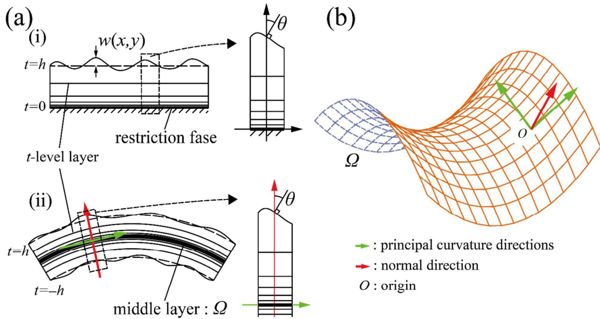
Figure 5| Schematic illustration of the model for describing the mechanical instability of gel sheet during free swelling. (a) The gel is treated as the combination of thin layers which are named t -level. In particular, the gel has the restriction face in the case of (i), and the gel passes through the process of the free swelling in the case of (ii). In both cases, \theta means the angle between the layer with the least deformity and the t -level layer. (b) The local coordinates on the middle layer, \Omega , of the free swelling gel. The green arrows correspond to the directions of the two principal curvatures, and the red arrow corresponds to the direction of the outward normal at the origin, O , on restriction phase.
