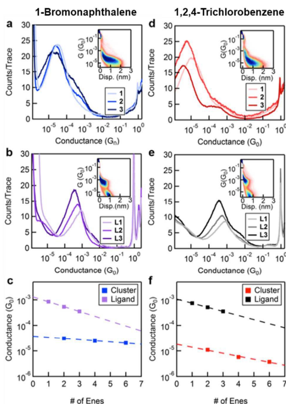
Fig. 2 Logarithmically-binned conductance histograms for 1-3 in (a) BrN and (d) TCB and L1-L3 in (b) BrN and (e) TCB. Insets in (a, d) and (b, e) are 2D histograms for 1 and L1 respectively. (c) and (f) Conductance peak values of the single molecule junctions for 1-3 and L1-L3 as a function of total number of “ene” units (e.g., 1 has 2 units while L1 has 1 unit) for measurements in BrN and TCB, respectively shown on a semi-log plot along with least-square linear fits. Marker size reflects the error in the Gaussian fits to the conductance histogram peaks.
