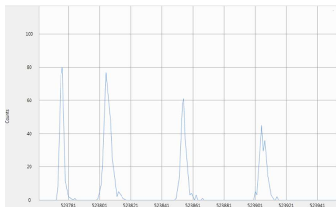
Figure 3. Zoomed in of four NP events at a dwell time of 50 \mu s. Particle concentration of 250,000 particles/mL
