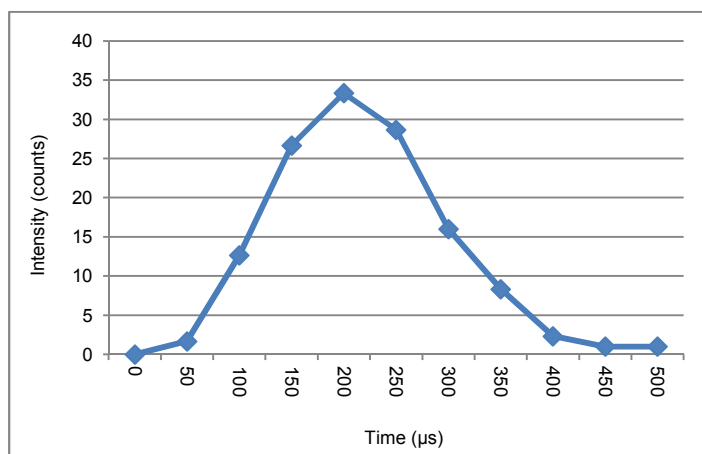
Figure 4. Raw data of a NIST SRM 8013 60 nm Gold Nanoparticle acquired at a dwell time of 50 \mu s
