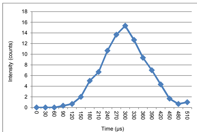
Figure 5. Raw data of a NIST SRM 8013 60 nm Gold Nanoparticle acquired at a dwell time of 30 \mu s
