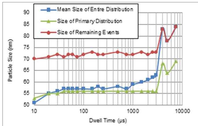
Effect of Dwell Time on Mean Particle Size Calculation for 250,000 particles/mL of 60 nm Au NPs nebulized at 300 \mu\text{L}/\text{min}
