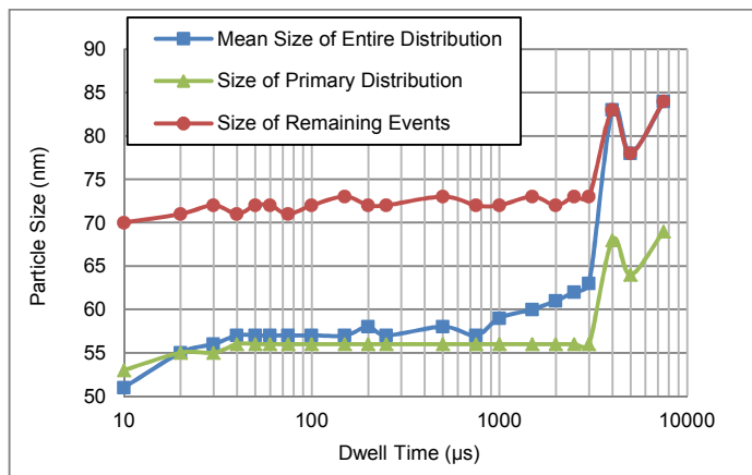
Figure 12. Effect of Dwell Time on Mean Particle Size Calculation for 250,000 particles/mL of 60 nm Au NPs nebulized at 300 \mu\text{L}/\text{min}
