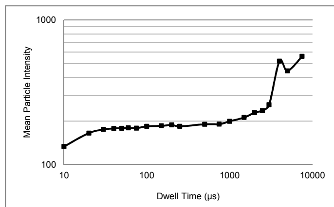
Figure 11. Effect of Dwell Time on Mean Particle Intensity for 250,000 particles/mL of 60 nm Au NPs nebulized at 300 \mu\text{L}/\text{min}
