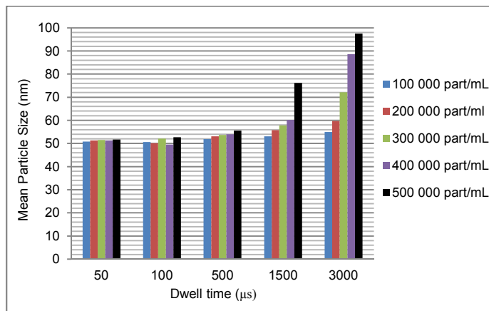
Figure 14. The effect of Dwell Time and NP concentration on particle sizing
