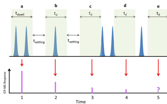
Figure 1. Effect of dwell and settling times on single particle measurements. a) 2 particles detected b) 1 single particle detected c) The leading edge of 1 particle detected d) The trailing edge of 1 particle detected e) No particles detected.
