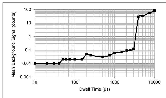
Figure 15. Effect of Dwell Time on Background Signal
