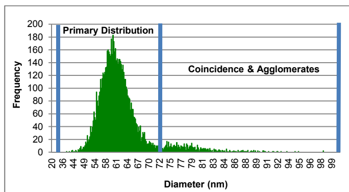
Figure 8. Size histogram of NIST SRM 8013 60 nm Gold Nanoparticles at a concentration of 250,000 particles/mL acquired at a dwell time of 50 \mu\text{s}
