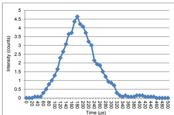
Figure 6. Raw data of a NIST SRM 8013 60 nm Gold Nanoparticle acquired at a dwell time of 10 \mu s
