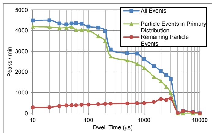
Figure 9. Particle Events vs Dwell Time for 250,000 particles/mL of 60 nm Au NPs nebulized at 300 \mu\text{L}/\text{min} . Data separated by grouping events in the primary distribution
