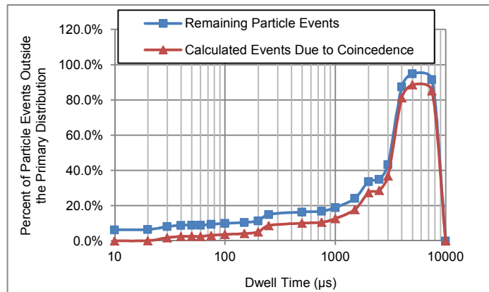
Figure 10. Percent of Particle Events Outside the Primary Distribution vs Dwell Time for 250,000 particles/mL of 60 nm Au NPs nebulized at 300 \mu\text{L}/\text{min}
