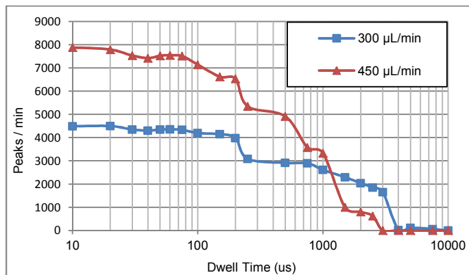
Figure 7. Particle Events vs Dwell Time for 250,000 particles/mL of 60 nm Au NPs nebulized at different flow rates
