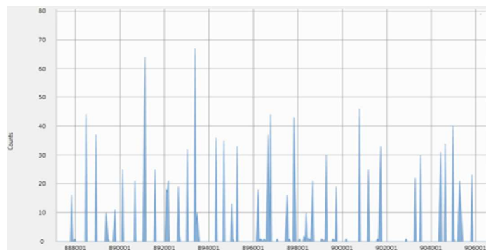
Figure 2. Zoomed in trace of NIST SRM 8013 60nm Gold Nanoparticle standard at a dwell time of 50 \mu s. Particle concentration of 250,000 particles/mL
