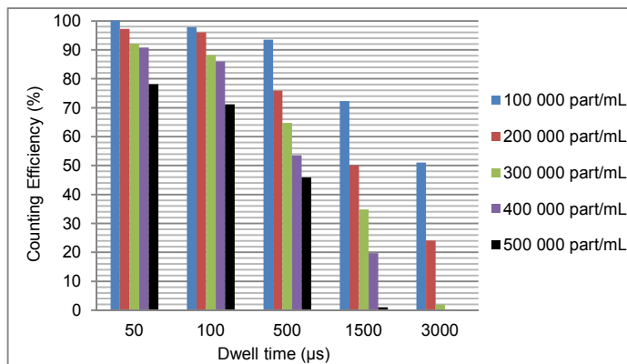
Figure 13. The effect of Dwell Time and NP concentration on particle counting.
