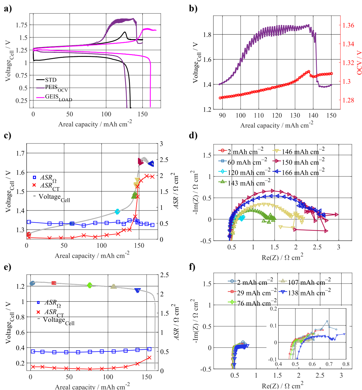
Figure 6: a) U - Q_{\text{areal}} dependence of a charge-discharge cycle for different characterization techniques STD, PEIS OCV and GEIS LOAD for ZIHFB with omitted zinc ions in posolyte (besides STD). b) OCV Cell dependence on Q_{\text{areal}} during PEIS OCV characterization. c) U - Q_{\text{areal}} dependence during GEIS LOAD characterization with evaluated ASR_{CT} and ASR_{\Omega} , colours used in the voltage cell evolution are linked to d) where EIS spectra are displayed with colour for corresponding Q_{\text{areal}} . Figures e) and f) represents the same as c) and d) , but for battery discharge. Experimental conditions: Std. negolyte composition, ZnI 2 omitted from posolyte (besides STD); Both electrolytes' volumes 0.07 dm 3 .
