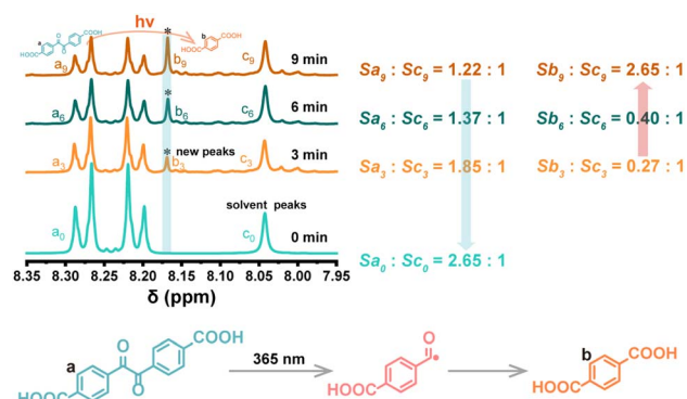
Fig. 2 Characterization of products after BS irradiation. ^1\text{H} NMR (400 MHz) spectra of BS in DMF- d_6 after different irradiation times using an external UV torch light ( 317.5 mW \text{cm}^{-2} ).
