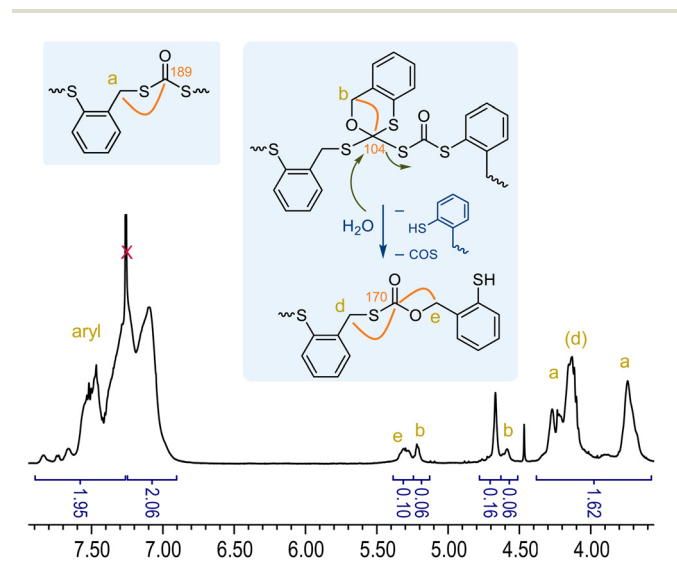
Fig. 1 ^1\text{H} NMR spectrum of pBOT (Table 1, entry 1) with assignments. The orange numbers refer to the measured ^{13}\text{C} chemical shifts (in ppm) found to couple with the assigned protons (orange lines). The proton signal for 'd' is overlapped by the 'a' signal. The green arrows indicate the presumed mechanism for orthocarbonate hydrolysis, showing the degradability of the side product repeat units.
