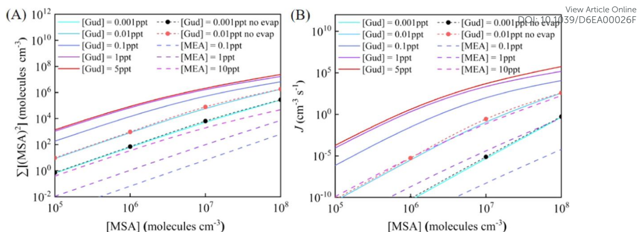
Figure 7. Variation of simulated steady-state MSA dimer concentration \Sigma[(\text{MSA})_2] (molecules cm -3 ) (A) and cluster formation rate J (cm -3 s -1 ) (B) with monomer concentration at 278.15 K and \text{CoagS} = 2.6 \times 10^{-3} \text{ s}^{-1} . Adapted from Liu et al., 2022 63 . Reproduced from ref. 63 with permission from the American Chemical Society, copyright 2022.
