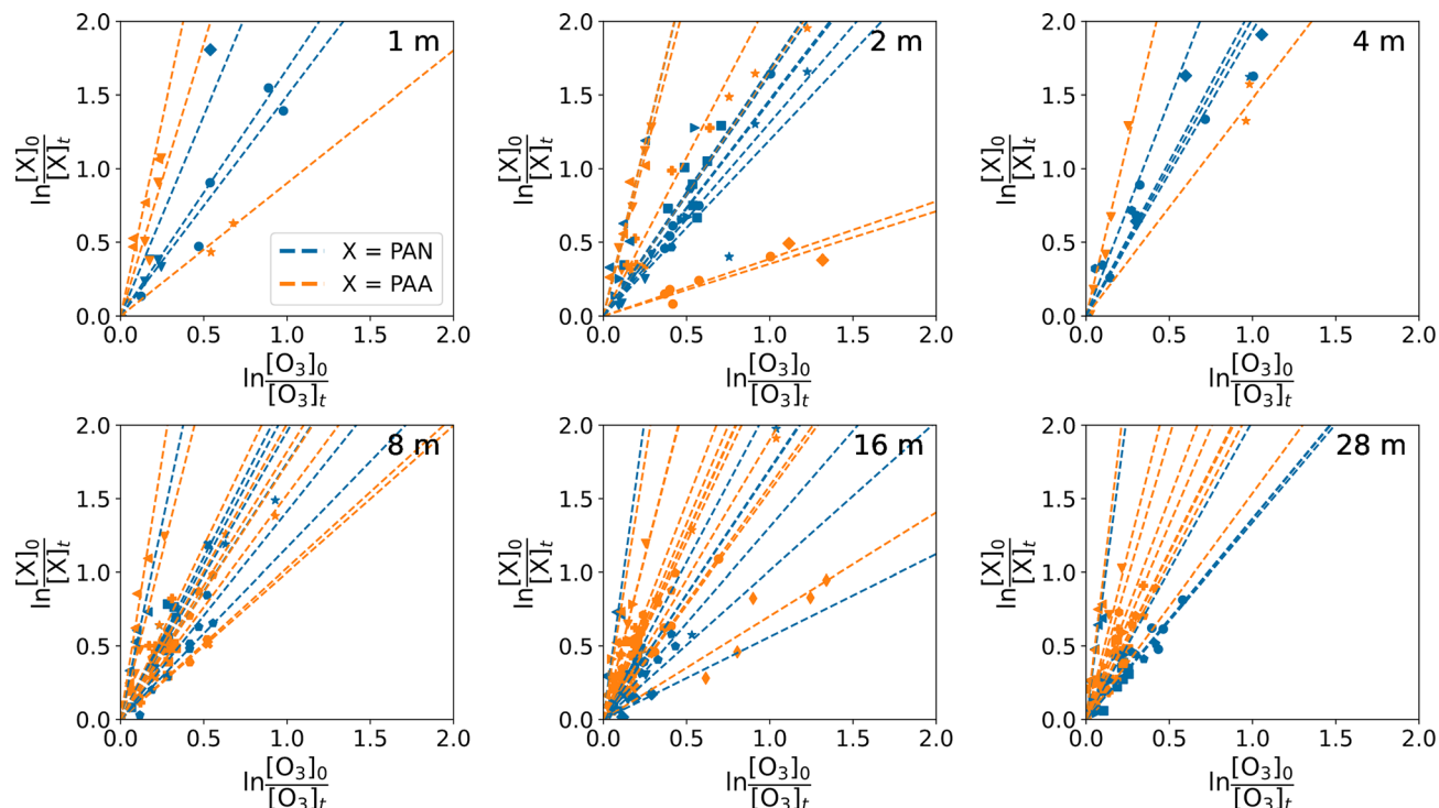
Fig. 4 Relative rates of PAN (blue) or PAA (orange) versus O_3 for individual nights at 1, 2, 4, 8, 16, and 28 m during the BAIRN-VIP campaign. Only data where r^2 > 0.8 is represented in this figure (see Section 3.2 for more details). A different symbol is used for each night.
