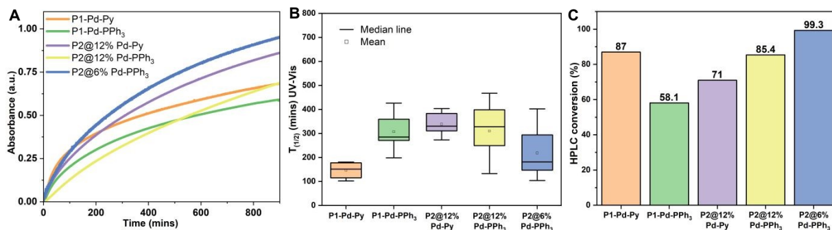
Figure 2. A) Kinetic profiles of encapsulated P1 and covalently attached P2 NPs in a pro-DNP ( 4 ) (100 μM) to DNP ( 5 ) conversion monitored by UV-Vis over time at \lambda = 400 nm in water at 37 °C using 30 μM of Pd; B) T_{1/2} comparison of the P1 and P2 NPs in the formation of DNP ( 5 ); T_{1/2} (time taken for 50 % formation of DNP ( 5 ) by UV-Vis, mean of multiple runs); C) HPLC conversion of DNP ( 5 ) after 24 h.
