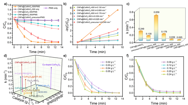
Fig. 3 (a) RhB degradation curves. (b) The corresponding fitted kinetics curves. (c) Histogram of first-order kinetic constant values in varied catalytic reaction systems. (d) Comparison of the intrinsic catalytic activity of the CNFs@CoMnO x -500 with reported catalysts towards PMS activation. Effect of (e) catalyst dosage, and (f) PMS concentration on RhB degradation.
