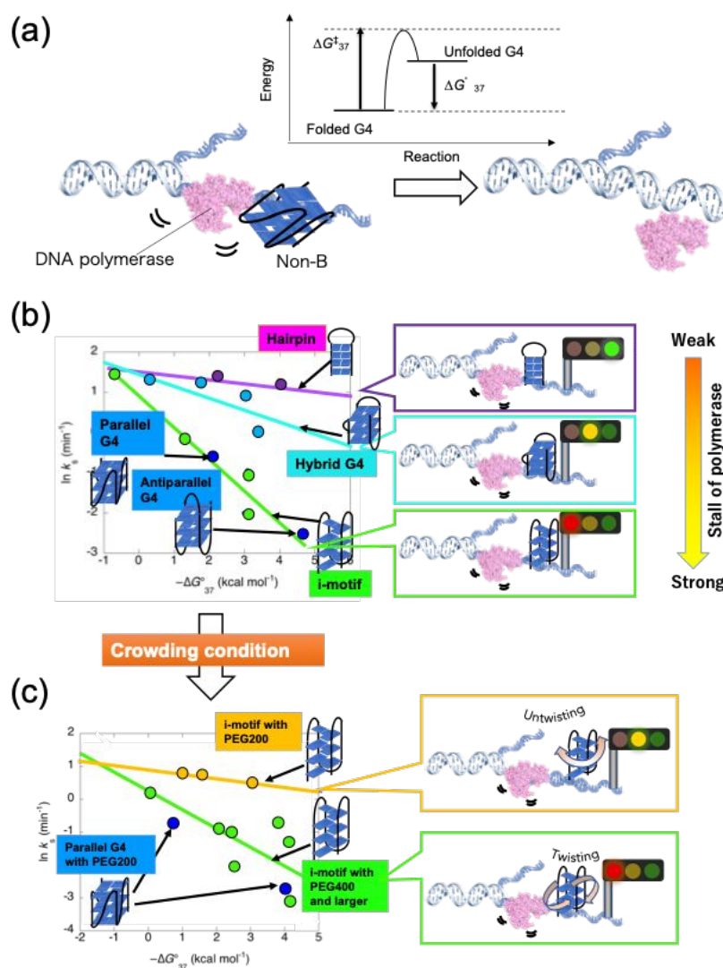
Fig. 8 Quantitative study of topology-dependent replication (QSTR) and its applications. (a) Parameters of the QSTR plot targeting the stability of the non-duplex ( -\Delta G^{\circ} ) and the activation energy required for polymerases to overcome the structure ( \Delta G^{\ddagger} ). (b, c) Plots of QSTR showing the relationship between the stability of the non-double helix structure and replication efficiency in the absence (b) or presence (c) of crowders at pH 6.0. 126, 127 The topology and dynamics dependency of replication inhibition is indicated by the difference in the slope of the QSTR plots. All the replication reactions were performed at 37 °C.
