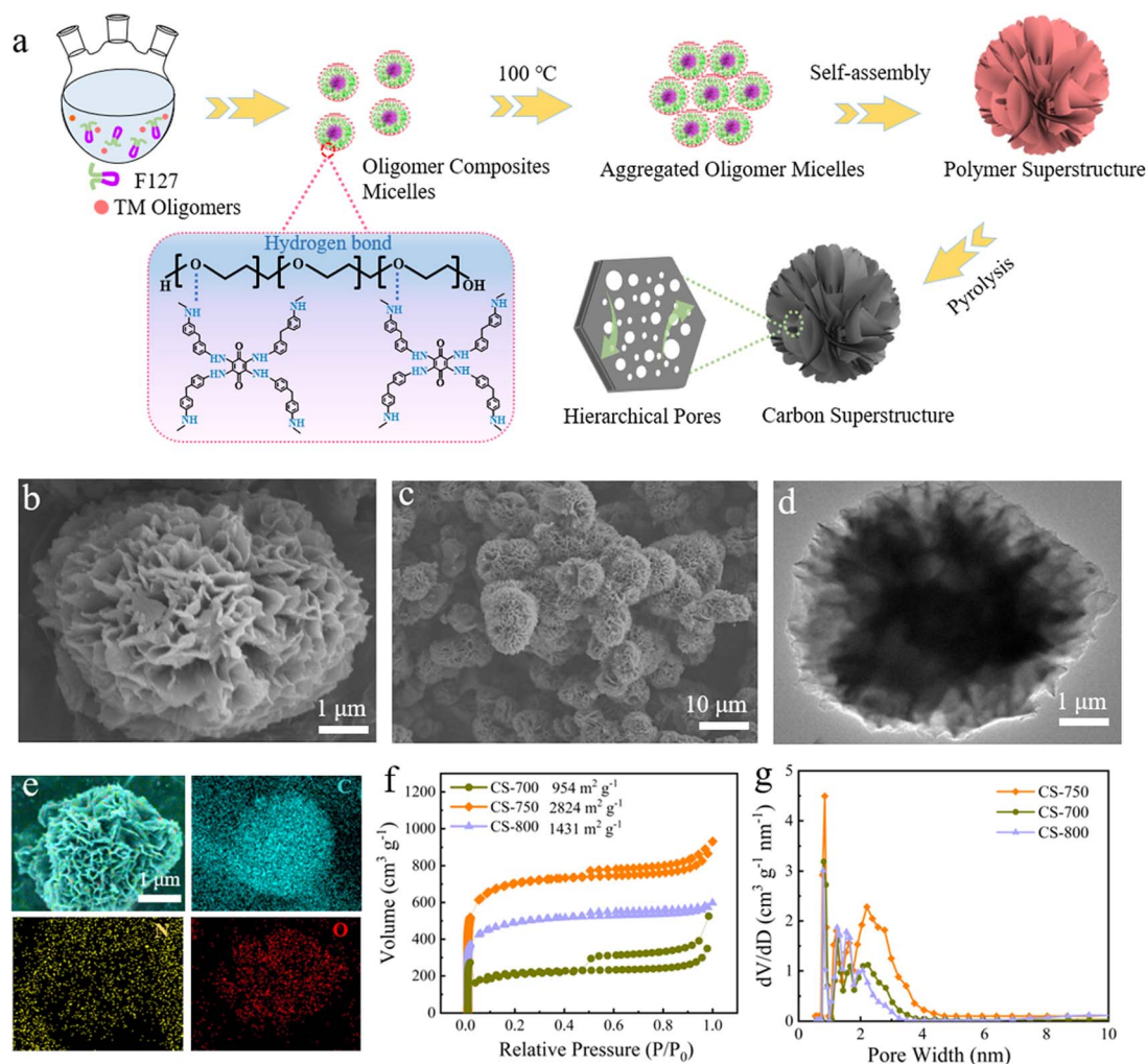
Fig. 1 (a) Schematic of the synthesis of carbon superstructures. (b and c) SEM images of CS-750. (d) TEM images of CS-750. (e) EDS mapping images of CS-750. (f) Nitrogen adsorption/desorption isotherms of CS-x. (g) Pore-size distribution curves of CS-x.
