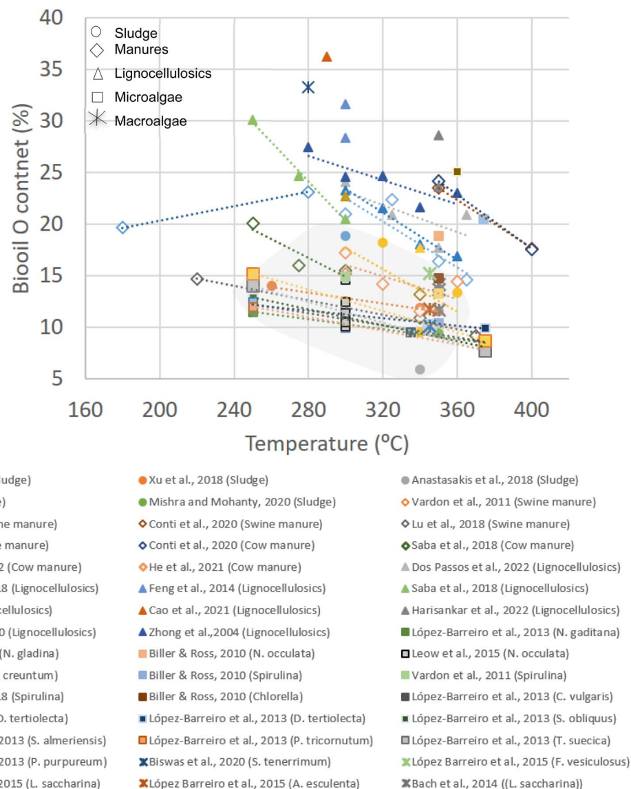
Fig. 8 Oxygen content in bio-oils reported by different authors. Trend lines were used for fitting experimental runs carried out at different temperatures in the same run (see in Table ESII†).
