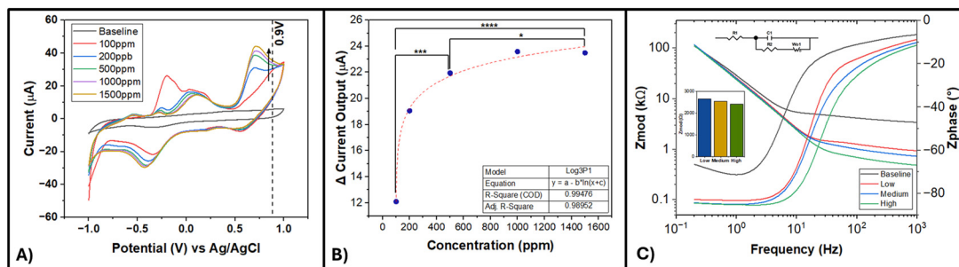
Fig. 2 A) Cyclic voltammetry performed from -1 V to +1 V for ethanol concentrations ranging from 100 ppm to 1500 ppm. B) Calibrated-dose-response curve for ethanol concentration ranging from 100–1500 ppm. C) Bode plots for ethanol detection from 100–1500 ppm. Extracted Z_{\text{mod}} change at 10 Hz depicting change in impedance low, medium and high concentrations of ethanol (inset).
