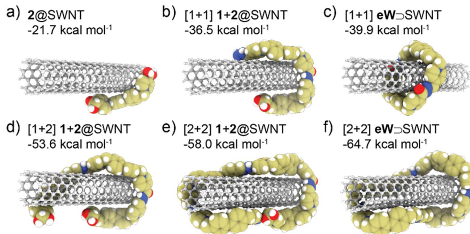
Fig. 6 Local minima and \Delta G_a^\circ values in \text{kcal mol}^{-1} computed at the \omega\text{B97X-3c}/\text{SMD}(\text{H}_2\text{O})//\text{GFN2}/\text{ALPB}(\text{H}_2\text{O}) level of theory, 16,17,22,23 for the potential aggregates formed by the association between a truncated hydrogen-capped section of a (6,5)-SWNT (ball-and-stick), and cyclic (c and f)/oligomeric (a, b, d and e) species arisen from the self-assembly of building blocks 1 and 2 (van der Waals spheres).
