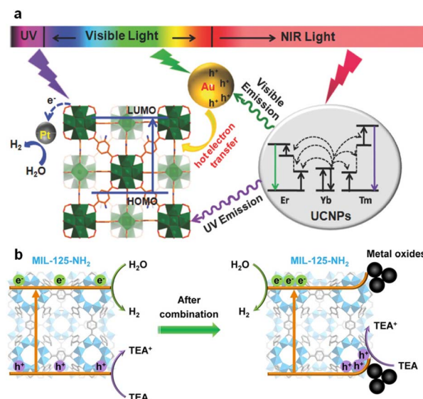
Fig. 10 (a) The light absorption region of UCNPs-Pt@MOF/Au. 87 Copyright 2018, John Wiley and Sons. (b) Schematic diagram of photocatalytic hydrogen production over \text{MIL-125-NH}_2 and metal oxides/ \text{MIL-125-NH}_2 . 93 Copyright 2022, John Wiley and Sons.
