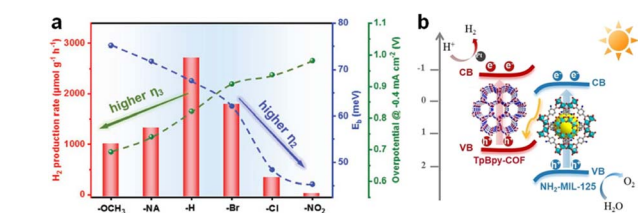
Fig. 9 (a) Photocatalytic \text{H}_2 production rate, E_b and overpotential in the HER of \text{UiO-66-NH}_2\text{@Pt@UiO-66-X} . 82 Copyright 2023, John Wiley and Sons. (b) Photocatalytic mechanism of the S-scheme heterojunction in \text{NH}_2\text{-MIL-125/TpBpy-COF} for overall water splitting. 84 Copyright 2025, John Wiley and Sons.
