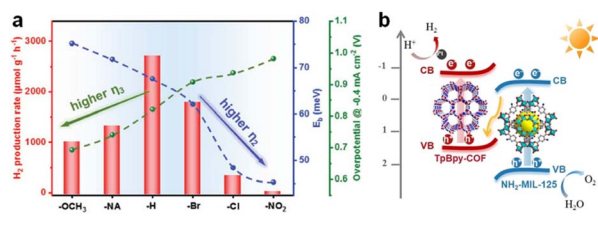
Fig. 9 (a) Photocatalytic H 2 production rate, E b and overpotential in the HER of UiO-66-NH 2 @Pt@UiO-66-X. 82 Copyright 2023, John Wiley and Sons. (b) Photocatalytic mechanism of the S-scheme heterojunction in NH 2 -MIL-125/TpBpy-COF for overall water splitting. 84 Copyright 2025, John Wiley and Sons.
