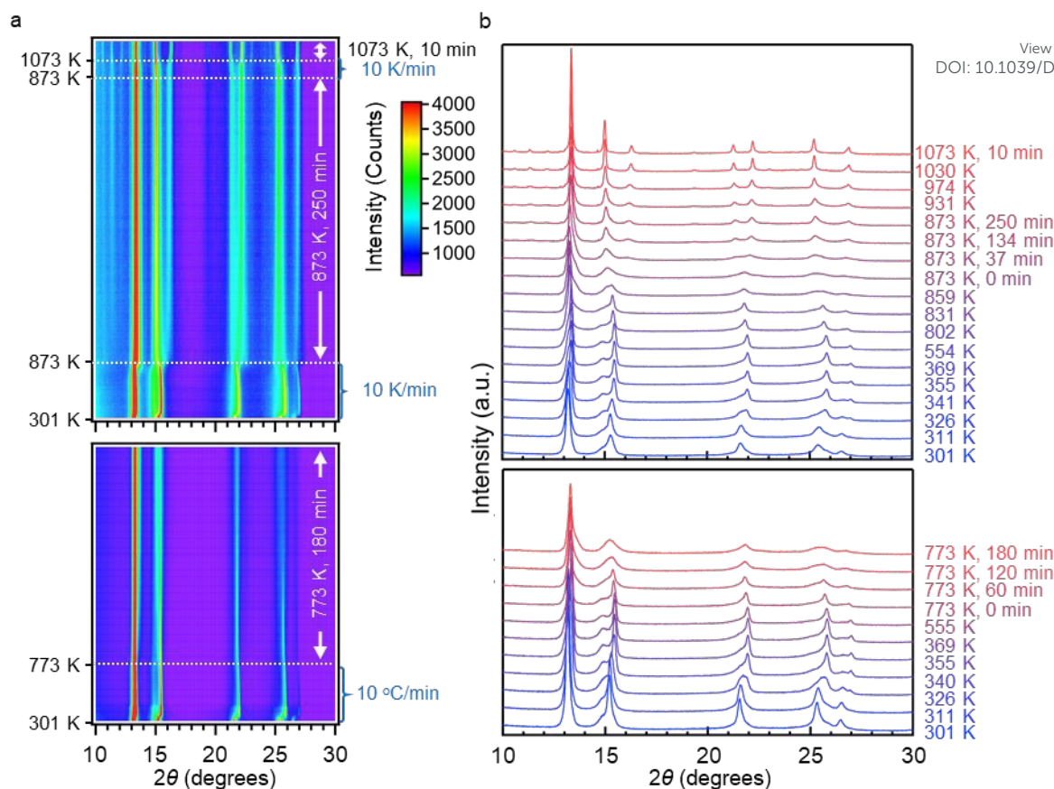
Fig. 5 (a) Two-dimensional plots of powder XRD patterns recorded during the reductive annealing of \text{PdIn}_x\text{Fe} NPs at the conditions marked with orange, red and green solid lines in Fig. 4a; (upper) heated to 873 K at 10 K/min, kept at 873 K for 250 min, heated to 1073 K at 10 K/min and kept at 1073 K for 10 min; (bottom) heated to 773 K at 10 K/min and kept at 773 K for 180 min. (b) Corresponding partial powder XRD patterns of the products.
