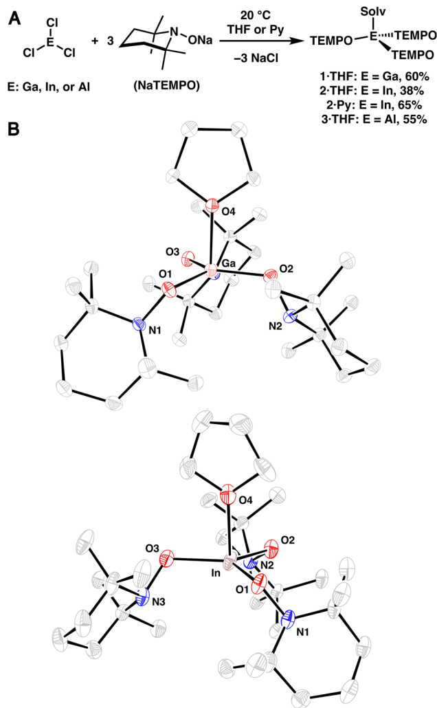
Fig. 1 (A) Synthesis of aminoxyl complexes 1·THF, 2·THF, 2·Py, and 3·THF. (B) SC-XRD structure of 1·THF (top) and 2·THF (bottom) with thermal ellipsoids shown at the 50% probability level. Hydrogen atoms are omitted for clarity.
