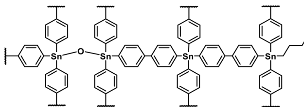
Fig. 1 Structure of Sn-OF-1. 20
