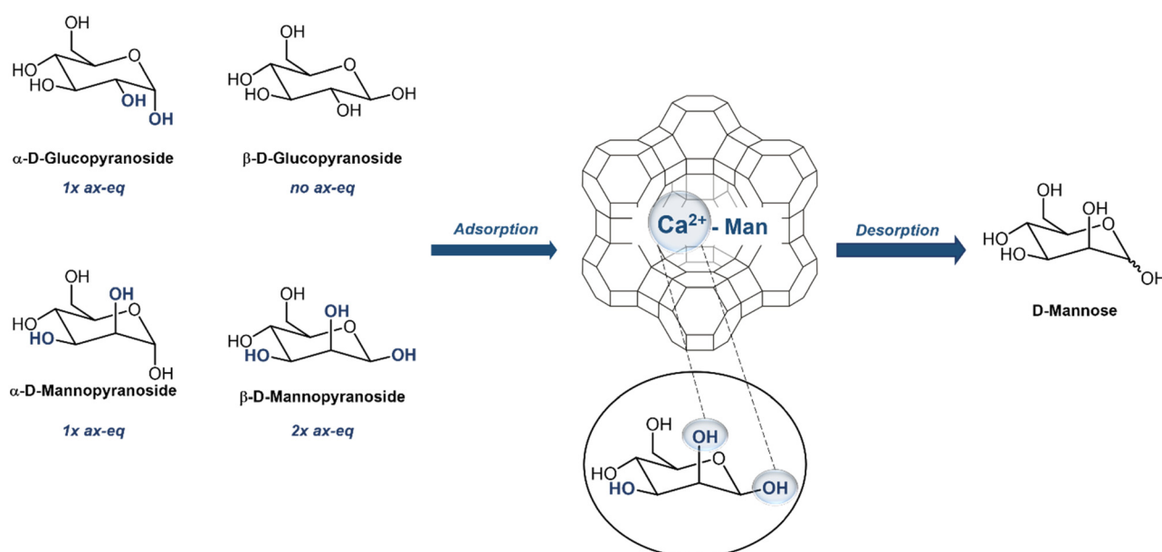
Fig. 2 Separation of D-Man via \text{Ca}^{2+} complexation in CaY zeolite.
