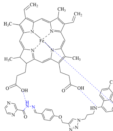
Fig. 8 Proposed binding of heme with H 37 . 54
