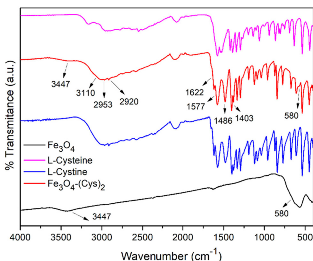
Fig. 3 FTIR spectra of \text{Fe}_3\text{O}_4 (black spectrum), \text{Fe}_3\text{O}_4 -(Cys) 2 (red spectrum), L-cystine (blue spectrum), and L-cysteine (magenta spectrum).
