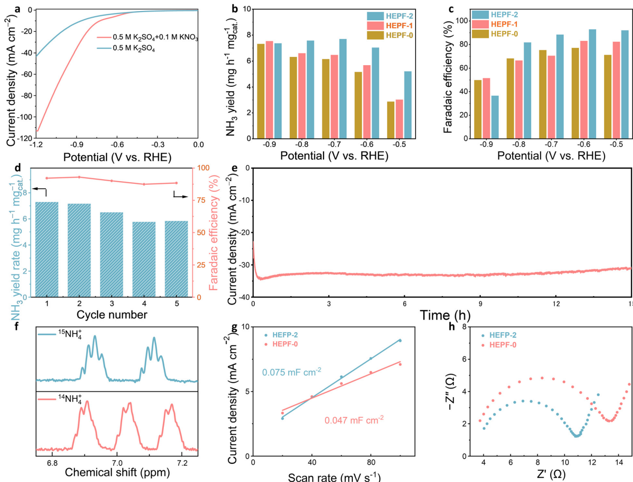
Fig. 4 (a) LSV curves for HEPF-2 in 0.5 M K 2 SO 4 electrolytes with and without KNO 3 , (b) NH 3 yield rates and (c) FE values of HEPF-0, HEPF-1 and HEPF-2 under different potentials. (d) NH 3 yield rates and FE values of HEPF-2 at -0.6 V vs. RHE for 5 cycles. (e) Long-term stability test of the HEPF-2 catalyst at -0.6 V vs. RHE in electrolyte with 0.1 M KNO 3 . (f) 1 H NMR spectra of NH 4 + prepared with K 15 NO 3 and K 14 NO 3 as nitrogen sources. (g) The C dl values of the HEPF-2 and HEPF-0 catalysts. (h) Nyquist plots of HEPF-2 and HEPF-0 catalysts.
