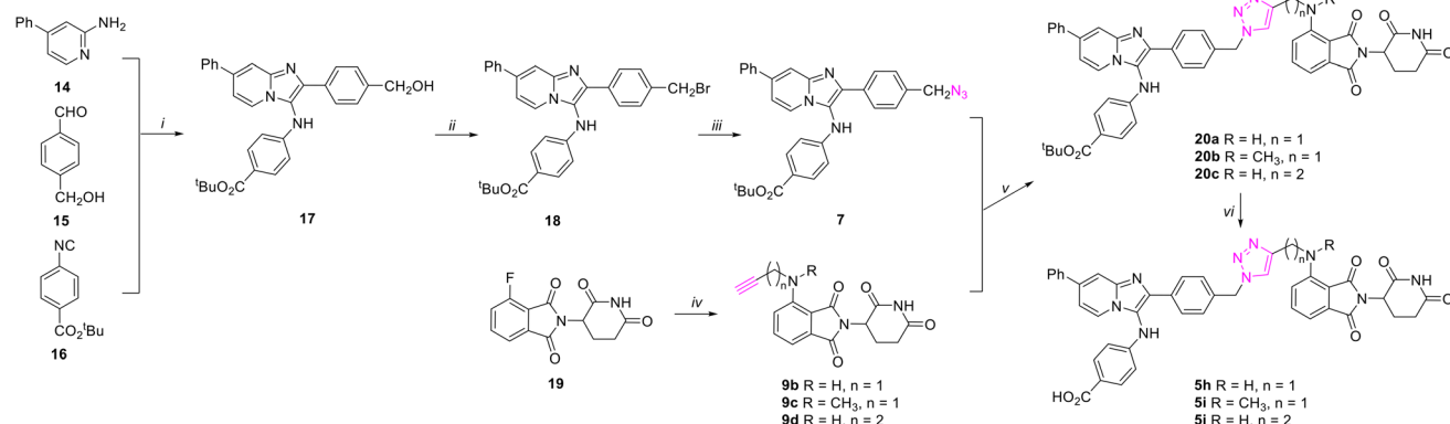
Scheme 3 Synthesis of compounds 5h–5j using key GBBR multi-component reaction and CuAAC “click” reaction. Reagents and conditions: (i) HOAc, MeOH; (ii) \text{CBr}_4 , \text{Ph}_3\text{P} , \text{CH}_3\text{CN} , rt; (iii) \text{NaN}_3 , \text{CH}_3\text{COCH}_3 , 55^\circ\text{C} ; (iv) amines (a, \text{CH}\equiv\text{CCH}_2\text{NH}_2 ; b, \text{CH}\equiv\text{CCH}_2\text{NHCH}_3 ; c, \text{CH}\equiv\text{CCH}_2\text{CH}_2\text{NH}_2 ), DMSO, 130^\circ\text{C} ; (v) TBTA, \text{CuSO}_4 \cdot 5\text{H}_2\text{O} , sodium L-ascorbate, DMSO, \text{H}_2\text{O} , rt. (vi) TFA, DCM.
