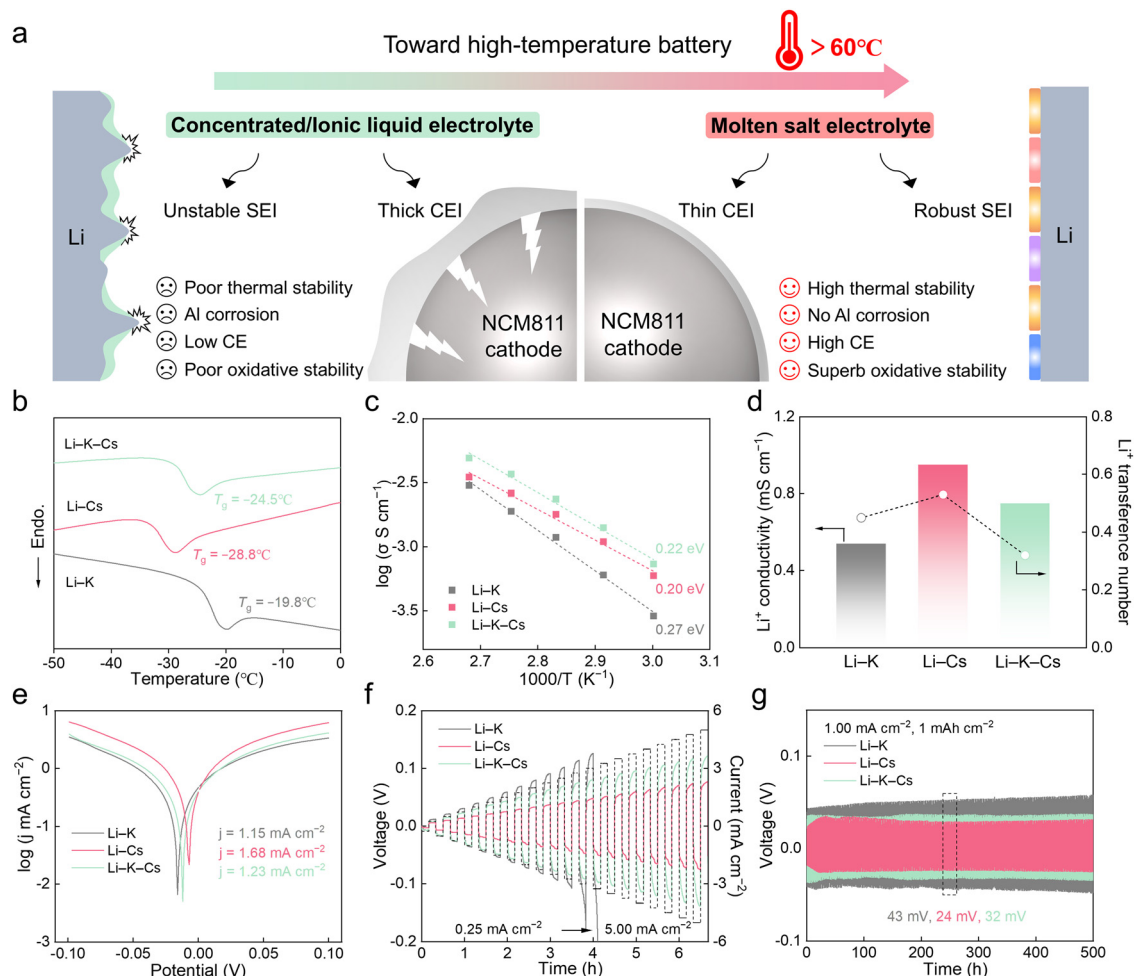
Fig. 1 Li + transport kinetics study in molten salt electrolytes. (a) Summary of the drawbacks and advantages of different electrolytes. (b) DSC curves of the three molten salts. (c) Ionic conductivity and activation energy calculation. (d) The true Li + conductivity and transference number at 80 °C. (e) Tafel plots and exchange current densities of three molten salts. (f) Rate performance of Li/Li symmetric cells at different current densities. (g) Galvanostatic cycling of Li/Li symmetric cells at 1.00 mA cm -2 with 1 mA h cm -2 .
