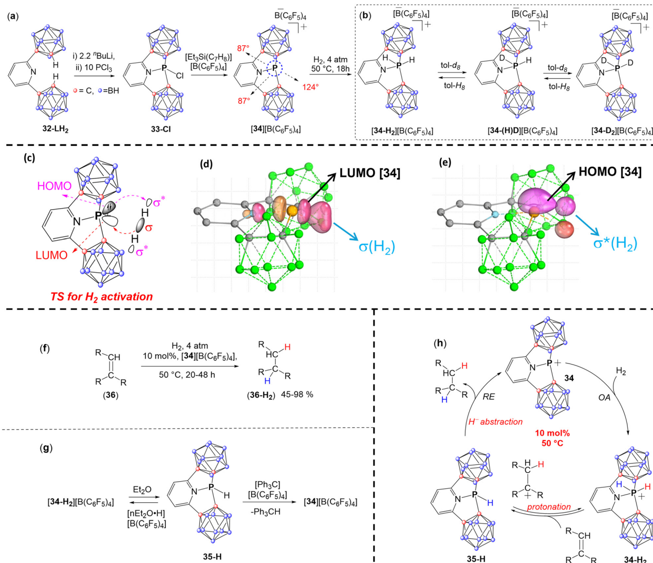
Fig. 13 Synthetic scheme for (a) the synthesis of [34][B(C_6F_5)_4] ; (b) the activation of dihydrogen by [34][B(C_6F_5)_4] and the exchange reaction between H-H bond by 34 ; (c) schematic representation to show electrophilically driven activation of the H-H bond by 34 ; (d) \sigma -bond of H_2 approaching the P-centre from the direction of the LUMO of 34 ; (e) followed by the interaction of the HOMO of the P-centre with the LUMO ( \sigma^* ) of H_2 ; (f) [34][B(C_6F_5)_4] catalyzed hydrogenation reactions of unsaturated C-C species; (g) equilibrium of [34][B(C_6F_5)_4] with 35-H and reaction of 35-H with [Ph_3C][B(C_6F_5)_4] ; and (h) the proposed catalytic cycle.
