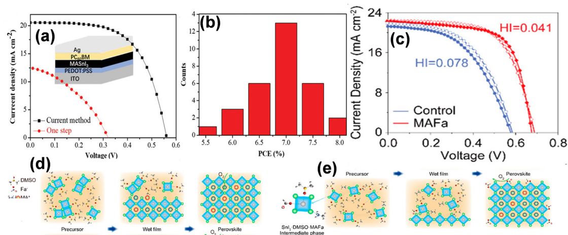
Fig. 4 (a) and (b) J–V curves and histograms of PCEs for 30 devices of MASnI 3 films, respectively. Reproduced with permission from ref. 54, copyright 2020, Wiley. (c) J–V curves of the control and MAFA-containing TPSCs. (d) and (e) Schematic of the crystallization process of the control and MAFA-derived perovskite films. Reproduced with permission from ref. 134, copyright 2023, ACS.
