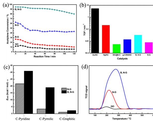
Fig. 10 (a) Catalytic reactivity evaluation of GO, B-G, N-G and B, N-G. The reactions were carried out at 150 °C, atmospheric pressure, a gas hourly space velocity (GHSV) of 36 h -1 , HCl/C 2 H 2 = 1.15/1 (volume ratio). (b) The TOFs for different catalysts: Au/AC, Hg/AC, SiC@N-C, g-C 3 N 4 /AC, B, N-G, N-G. (c) E_{\text{ads}} of HCl on different types of active sites in N-G and B, N-G. C-pyridine: the carbon atoms bonded with pyridinic N species. C-pyrrolic: the carbon atoms bonded with pyrrolic N species. C-graphitic: the carbon atoms bonded with graphitic N species. (d) TPD profile of HCl on GO, N-G and B, N-G. 90 Reproduced from ref. 90 with permission from American Chemical Society. Copyright 2015.
