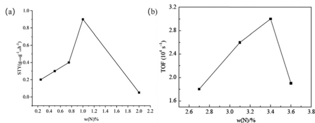
Fig. 9 (a) Space time yield of VCM of xNPCs with various ratios of melamine and PVC ( x = 0.25, 0.50, 0.75, 1.00, 2.00 ). The reaction conditions were 220 °C, GHSV of C 2 H 2 = 60 h -1 , HCl/C 2 H 2 volume ratio = 1.2; 62 reproduced from ref. 62 with permission from American Chemical Society, Copyright 2022. (b) The relationship between nitrogen content and TOF of N-OMC-Ox. 74 Reproduced from ref. 74 with permission from Elsevier, Copyright 2016.
