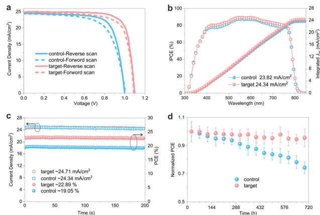
Fig. 4 (a) J - V curves measured in reverse and forward scan modes for the champion control and target PSCs. (b) IPCE (left axis) and corresponding integrated J_{\text{SC}} (right axis) for the control and target PSCs. (c) Stabilized efficiency after maximum power point tracking (MPPT) of the control and target devices for 200 s. (d) Normalized PCE of devices based on the control and target films in 30 days under continuous one-sun illumination in a \text{N}_2 environment at a room temperature of 25 ^{\circ}\text{C} .
