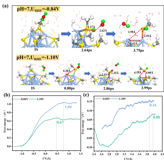
Fig. 1 (a) Schematic of local structures formed during ^*\text{H} adsorption onto the S site and during Ag–S bond breaking in \text{Ag}_{25}(\text{SR})_{18} at U_{\text{RHE}} = -0.84 \text{ V} and -1.10 \text{ V} . (b) Integral free energy curves for ^*\text{H} adsorption and (c) Ag–S bond breaking at U_{\text{RHE}} = -0.84 \text{ V} and -1.10 \text{ V} , respectively. The Ag, S, C, O and H atoms are shown as pale blue, yellow, grey, red and white spheres, respectively. The H from the attacking \text{H}_2\text{O} is colored in green.
