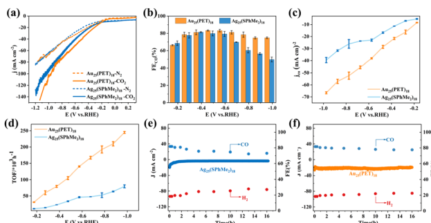
Fig. 4 Electrocatalytic CO 2 RR performance in a CO 2 flow cell with 1 M KOH electrolyte. (a) LSV curves of Ag 25 (SphMe 2 ) 18 and of Au 25 (PET) 18 , each in N 2 -saturated or CO 2 -saturated 1 M KOH electrolyte. (b) Faradaic efficiency of CO (FE CO ). (c) fractional current density of CO ( j CO ), and (d) turnover frequency (TOF) of CO for Ag 25 and Au 25 at indicated potentials. (e) and (f) Tests of long-term stability of (e) Ag 25 and (f) Au 25 in the CO 2 RR at −0.38 V.
