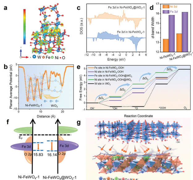
Fig. 5 (a) Charge density difference of \text{Ni-FeWO}_4\text{@WO}_3\text{-1} . (b) Plane-average electron difference diagram of the interface between \text{Ni-FeWO}_4\text{@WO}_3\text{-1} . (c) Projected DOS of Fe 3d in \text{Ni-FeWO}_4\text{-1} and \text{Ni-FeWO}_4\text{@WO}_3\text{-1} . (d) The d-band widths of Fe 3d and Ni 3d in \text{Ni-FeWO}_4\text{-1} and \text{Ni-FeWO}_4\text{@WO}_3\text{-1} . (e) Free energy profiles of different OER intermediates at 0 V for the Fe site. (f) Variation of the d-band widths of Fe 3d. (g) Schematic illustration of the electron barrier layer for the protection of Fe and Ni sites in \text{Ni-FeWO}_4\text{@WO}_3 . Reproduced with permission of ref. 71 copyright 2023, Wiley-VCH.
