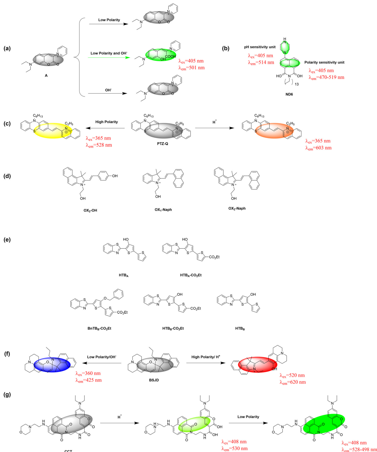
Fig. 6 Fluorescent probes for detecting polarity and pH.
