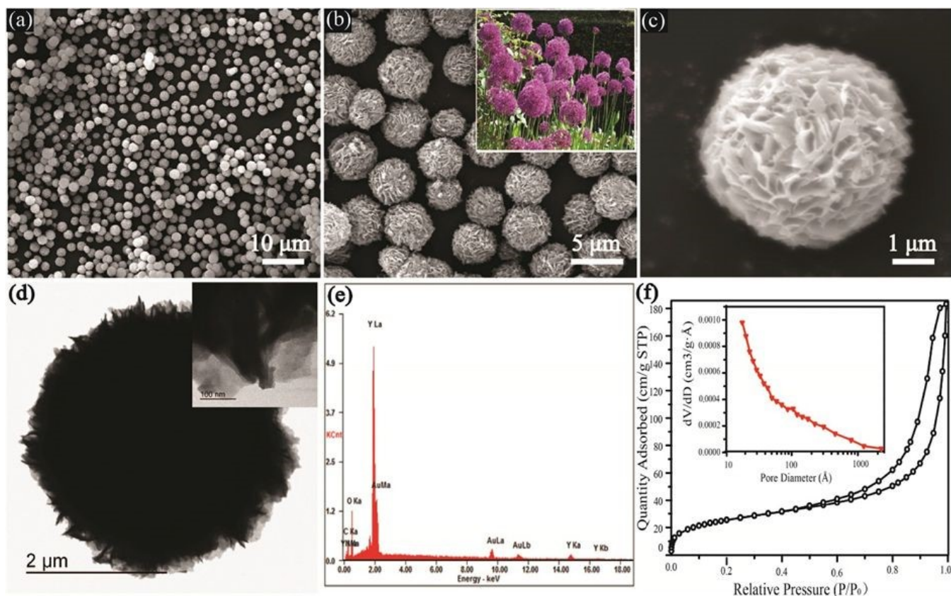
1 Fig 1. SEM and TEM images of as-prepared Y-MOFs samples at 120 °C for 24 h: (a–c) low- and 2 high-magnification SEM images (inset in (b) is the photo of allium giganteum) [26]; (d) low- and 3 high-magnification TEM images; (e) EDX spectrum [26]; (f) Nitrogen adsorption/desorption 4 isotherms of Y-MOFs: 10%Eu 3+ (inset is pore size distribution) [31]. 5
