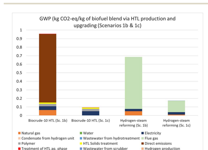
Fig. 8 LCA of HTL biocrude production and upgrading for Scenarios 1b and 1c. Scenario 1b: total value of GWP metric is 0.75 kg CO 2 -eq. per kg biocrude (or 0.02 kg CO 2 -eq. per MJ biocrude) and 1.64 kg CO 2 -eq. per kg (or 0.04 kg CO 2 -eq. per MJ) of fuel blend (diesel, naphtha), Scenario 1c: 0.07 kg CO 2 -eq. per kg biocrude (or 0.002 kg CO 2 -eq. per MJ biocrude) and 0.27 kg CO 2 per kg (or 0.01 kg CO 2 -eq. per MJ) of fuel blend (diesel, naphtha). Impacts of hydrotreatment/hydrocracking are not shown as they are negligible.
