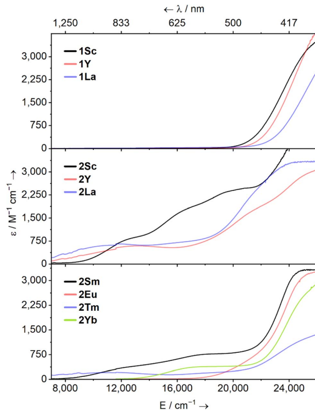
Fig. 2 Solution UV-Vis-NIR spectra of [M(\text{NHA}^{\text{iPr}_6})(\text{l})] ( 1M , M = Sc, Y, La; top) and [M(\text{NHA}^{\text{iPr}_6})] ( 2M , middle, M = Sc, Y, La; bottom, M = Sm, Eu, Tm, Yb) – as 1 mM solutions in \text{Et}_2\text{O} between 7000–26 000 \text{cm}^{-1} (1429–385 nm) at ambient temperature.
