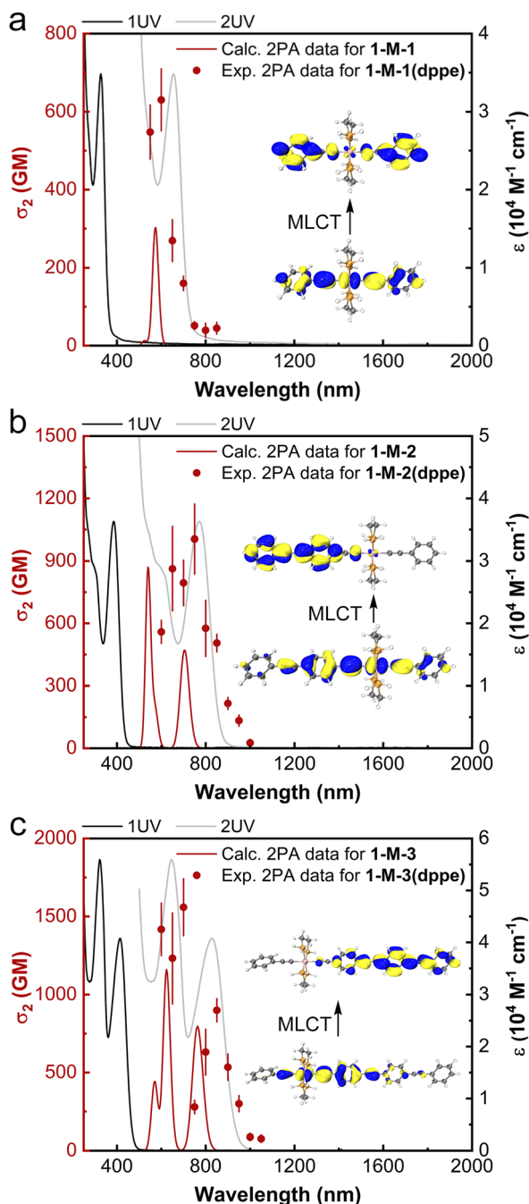
Fig. 5 Calculated 2PA cross-sections of 1-M-n ( n = 1-3 ) (red traces), experimental 2PA cross-sections of 1-M-n(dppe) ( n = 1-3 ) (red circles), linear absorption spectra of 1-M-n(dppe) ( n = 1-3 ) (black traces), and plots of the UV/Vis spectrum as a function of twice the wavelength (light gray traces). Insets: the metal-to-ligand charge transfer (MLCT) corresponding to the calculated low-energy 2PA maxima.
