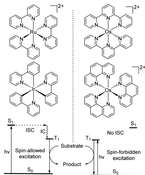
Fig. 4 Photocatalysis via conventional S_0 to S_1 absorption and spin-allowed excitation and spin-forbidden S_0 to T_1 absorption (ISC = intersystem crossing and IC = internal conversion).
