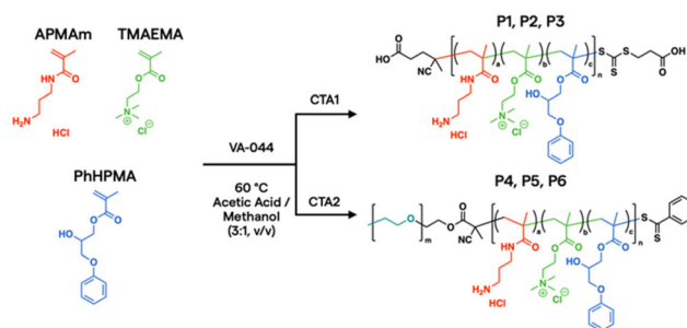
Scheme 1 RAFT synthesis of multimonomeric polyelectrolytes.
